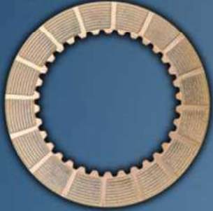
PARK BRAKE BRONZE DISC 315 SG/SJ
