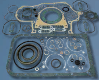
GASKET KIT FULL BF6L913
